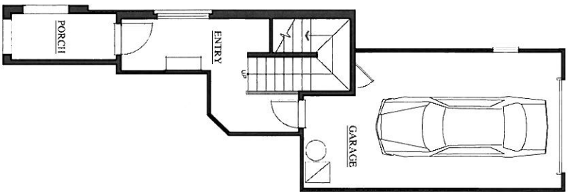
First Floor (Lower/Garage Level)
